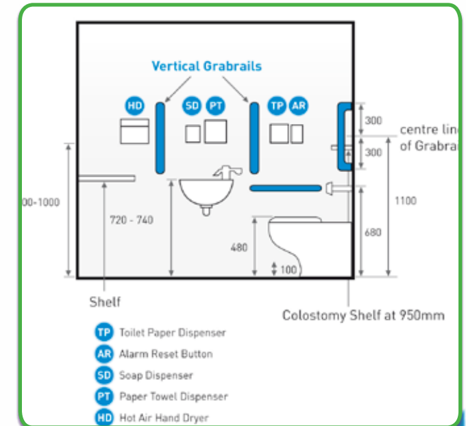
Figure 25 – Layout of an accessible toilet
