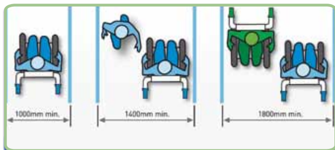
Figure 5 – Access widths for wheelchair users
