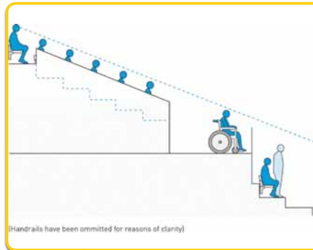
Figure 19 – An acceptable viewing standard for mid-tier wheelchair-user spaces (front of vomitory and surrounding non-disabled spectators)
