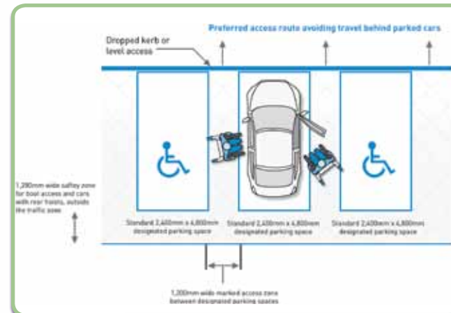
Figure 3 – Accessible parking spaces
