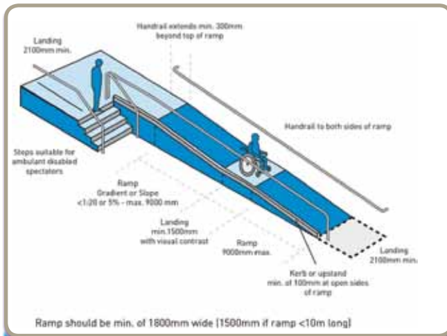
Figure 14 – A ramp with minimum widths, gradients and levels
