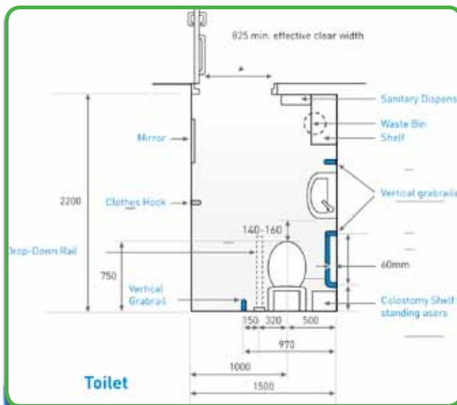
Figure 26 – Layout of an accessible toilet
