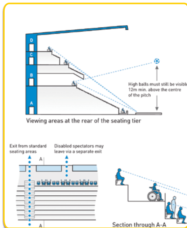
Figure 21 – Sightlines from elevated viewing positions
